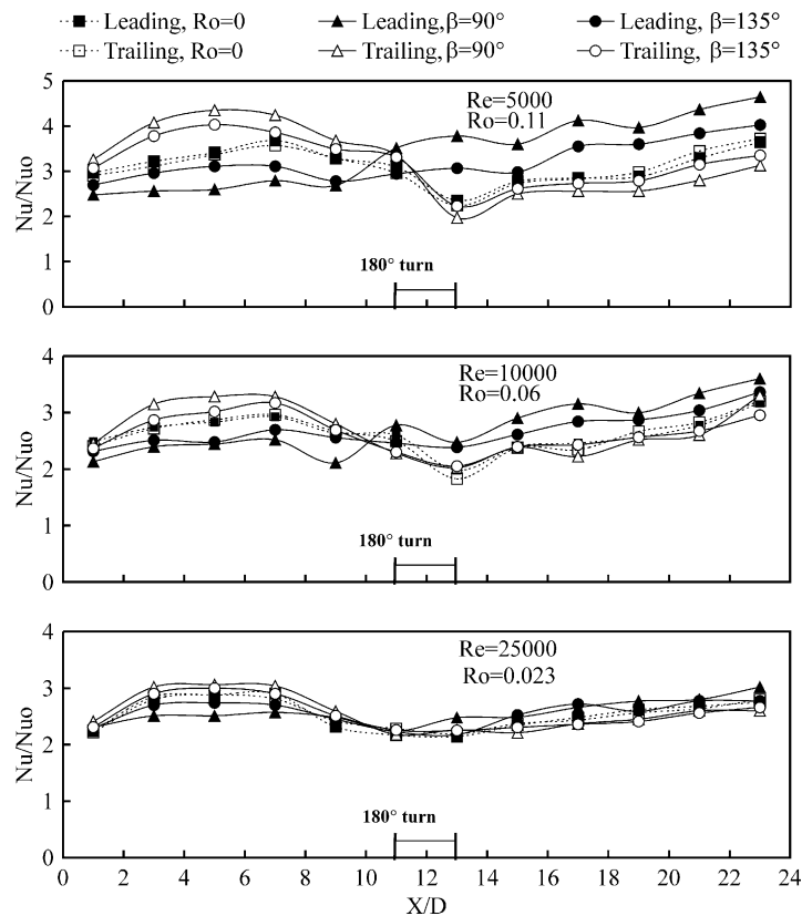
Fig. 8. Regional Nusselt number ratio for case (e).
