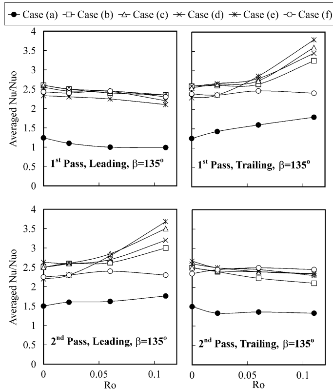
Fig. 11. Averaged Nusselt number ratio on leading and trailing surfaces for \beta = 135^\circ .
