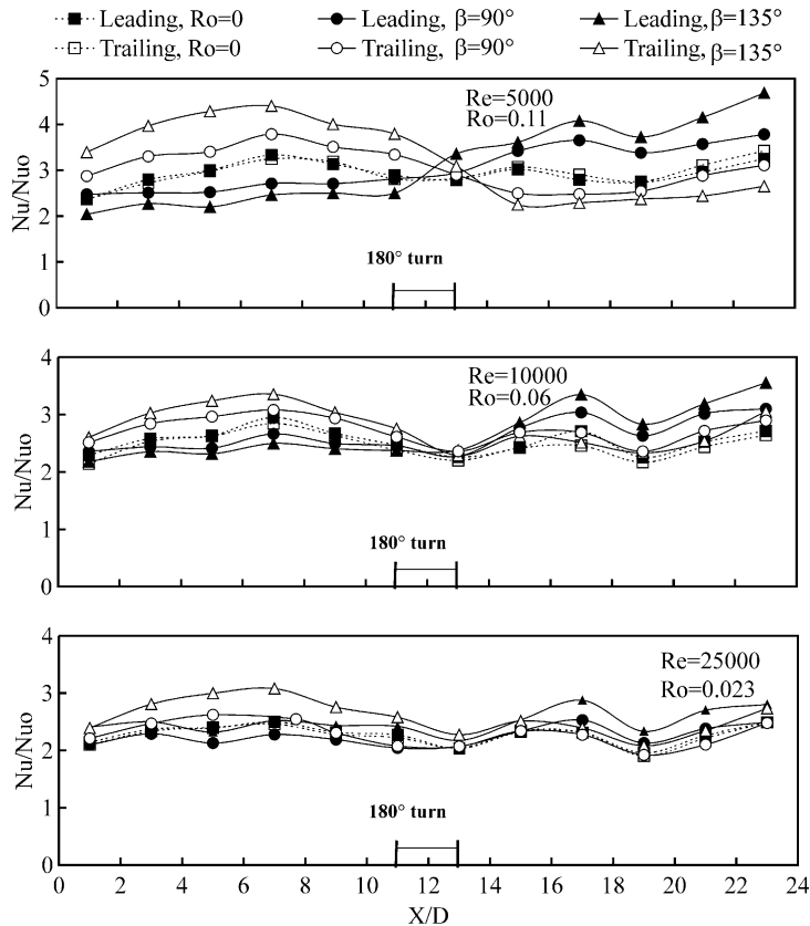
Fig. 6. Regional Nusselt number ratio for case (c).
